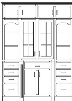
Hutch 3 5' wide, 7'2" high
